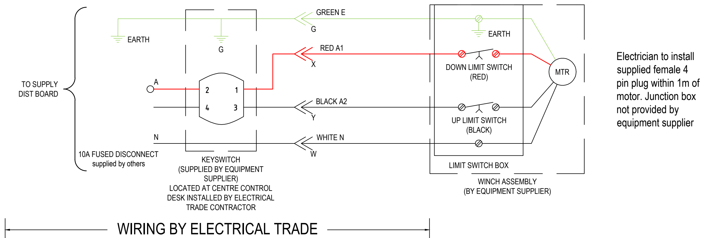
BASKETBALL WINCH, CURTAIN WINCH & CRICKET NETS TYPICAL WIRING SCHEMATICS NTS
