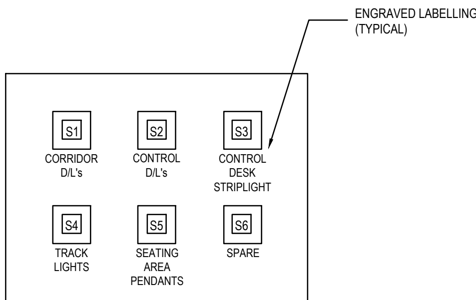
MASTER LIGHTING CONTROL PANEL (LSP-M) (LOCATED AT MAIN CONTROL DESK) REFER NOTE 3
