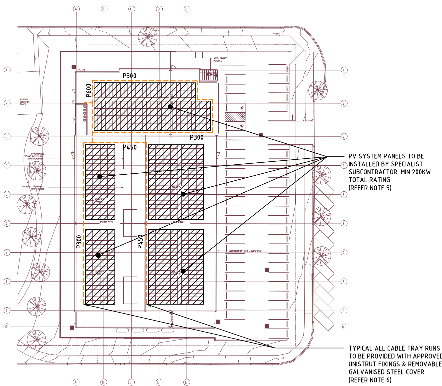
ROOF LEVEL PV SYSTEM GENERAL ARRANGEMENT PLAN SCALE 1:500
