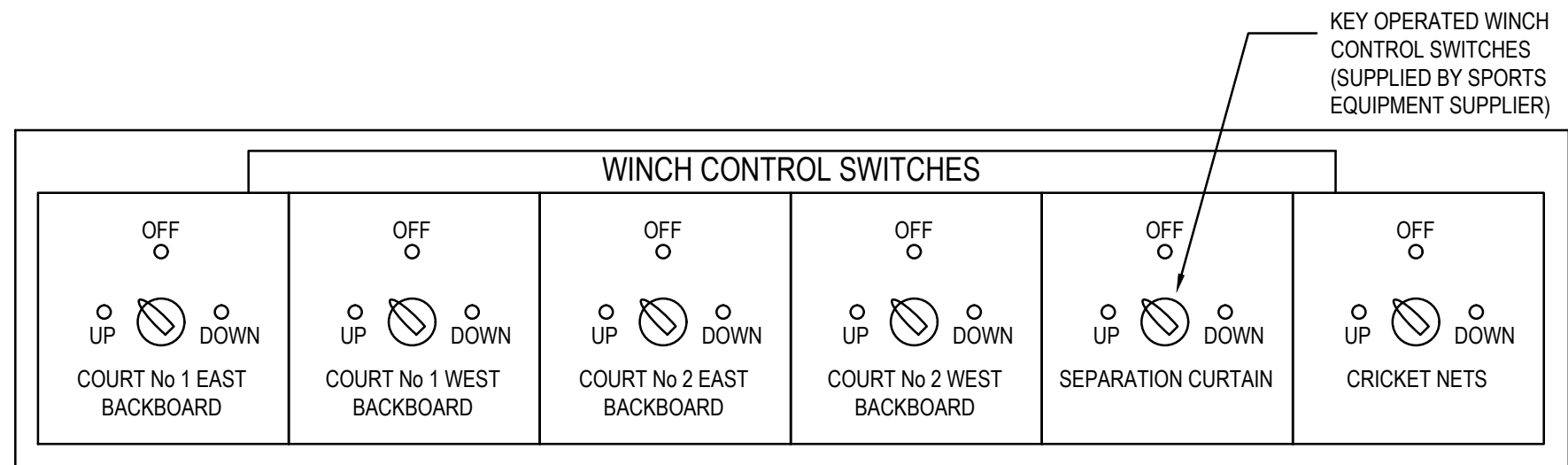
WINCH CONTROL PANEL (LOCATED AT MAIN CONTROL DESK)
