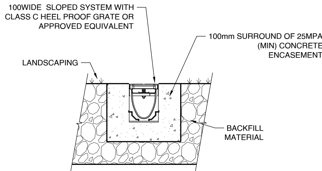
SECTION VIEW
