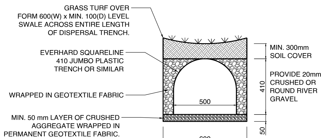
TYPICAL LEVEL SPREADER DISPERSAL TRENCH CROSS-SECTION N.T.S
