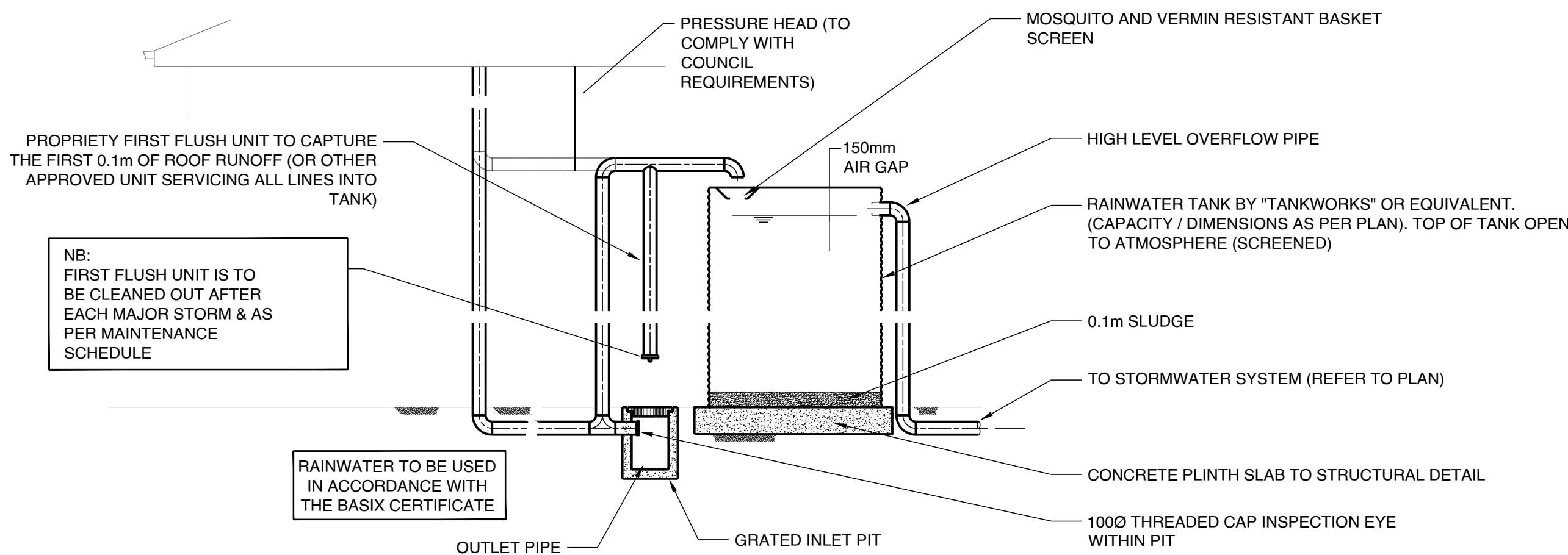
TYPICAL ABOVE GROUND RAINWATER STORAGE TANK
