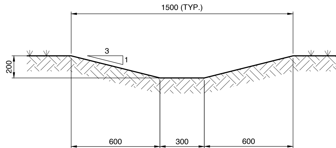
SECTION VIEW
