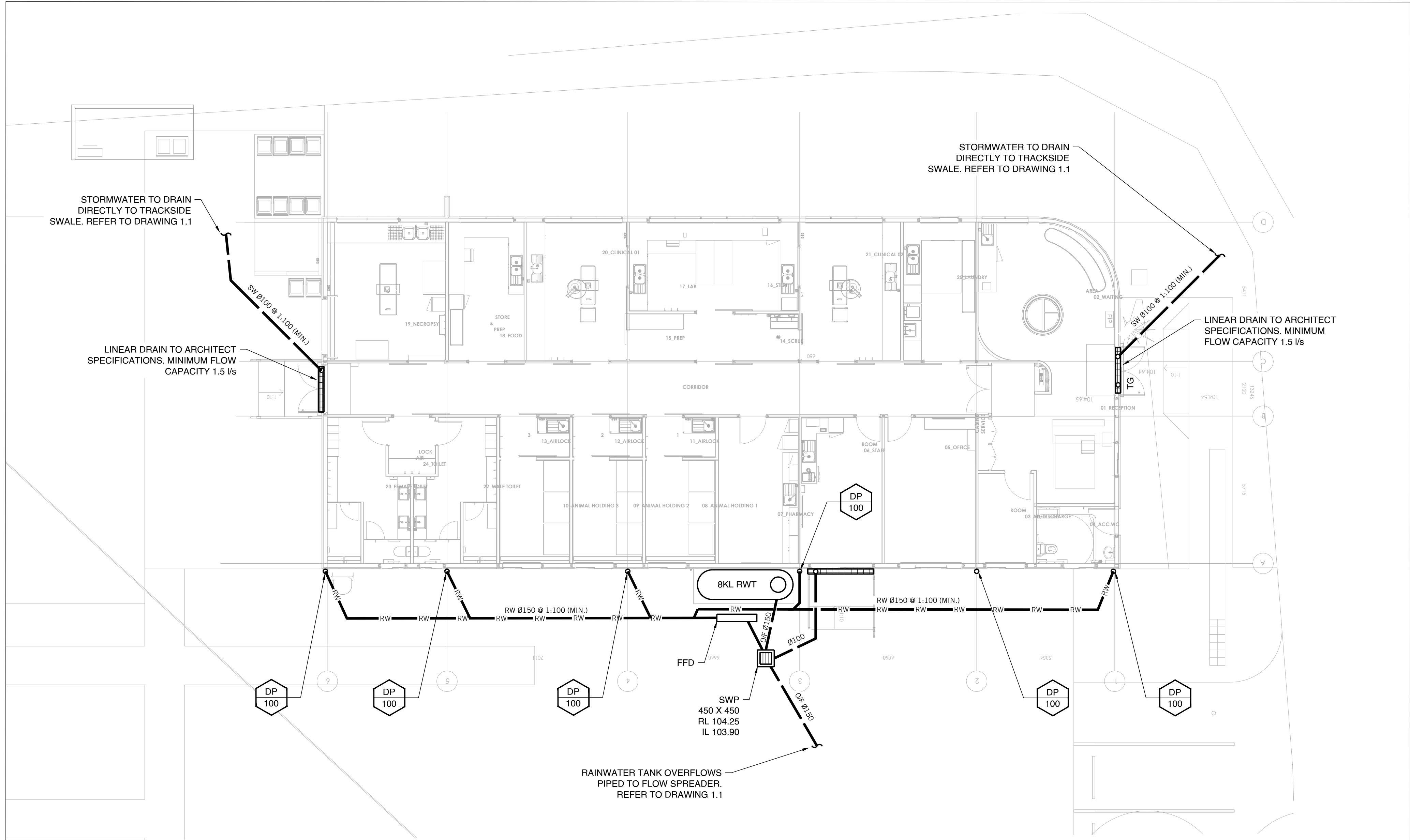
BUILDING LAYOUT
