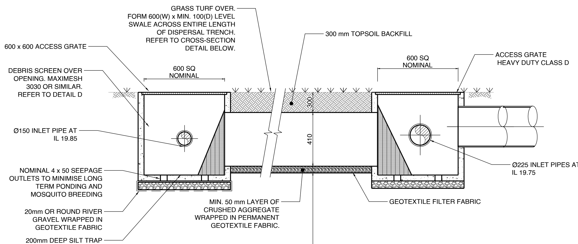
TYPICAL LEVEL SPREADER DISPERSAL TRENCH LONGITUDINAL SECTION N.T.S
