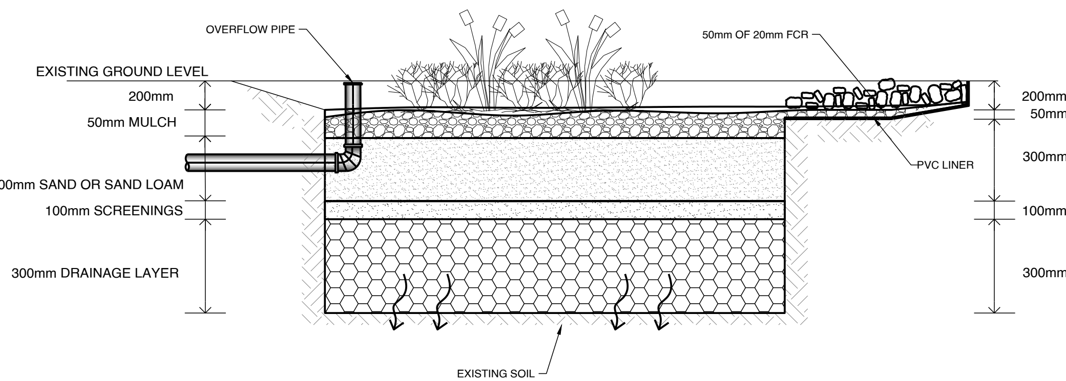
TYPICAL RAINGARDEN N.T.S
