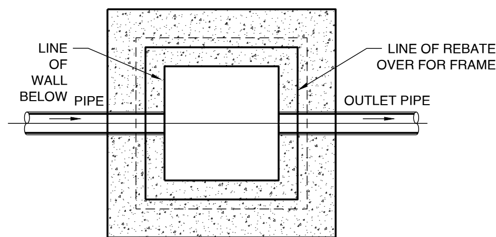
PLAN WITHOUT GRATE
