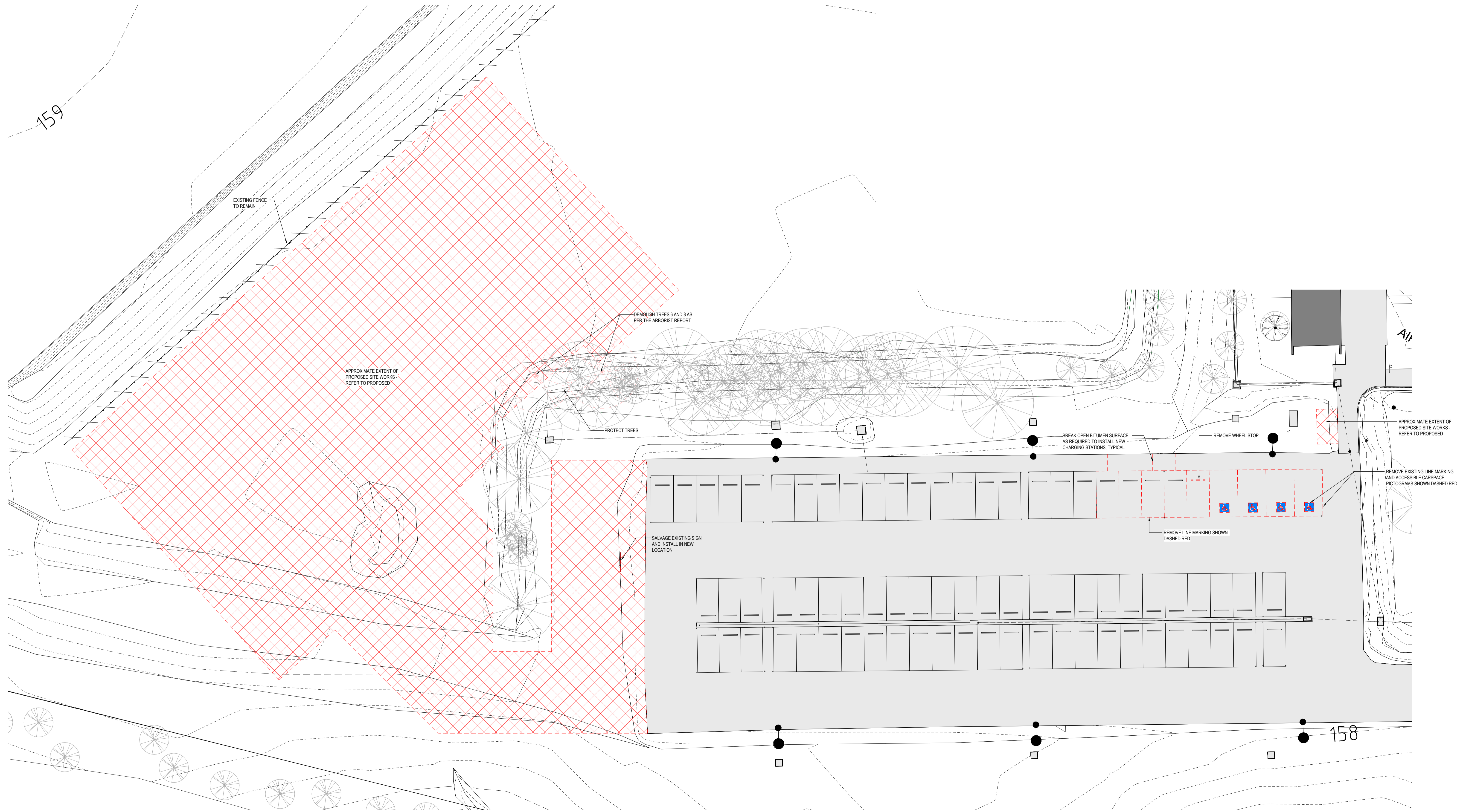
SITE PLAN - DEMOLITION SCALE 1:200
