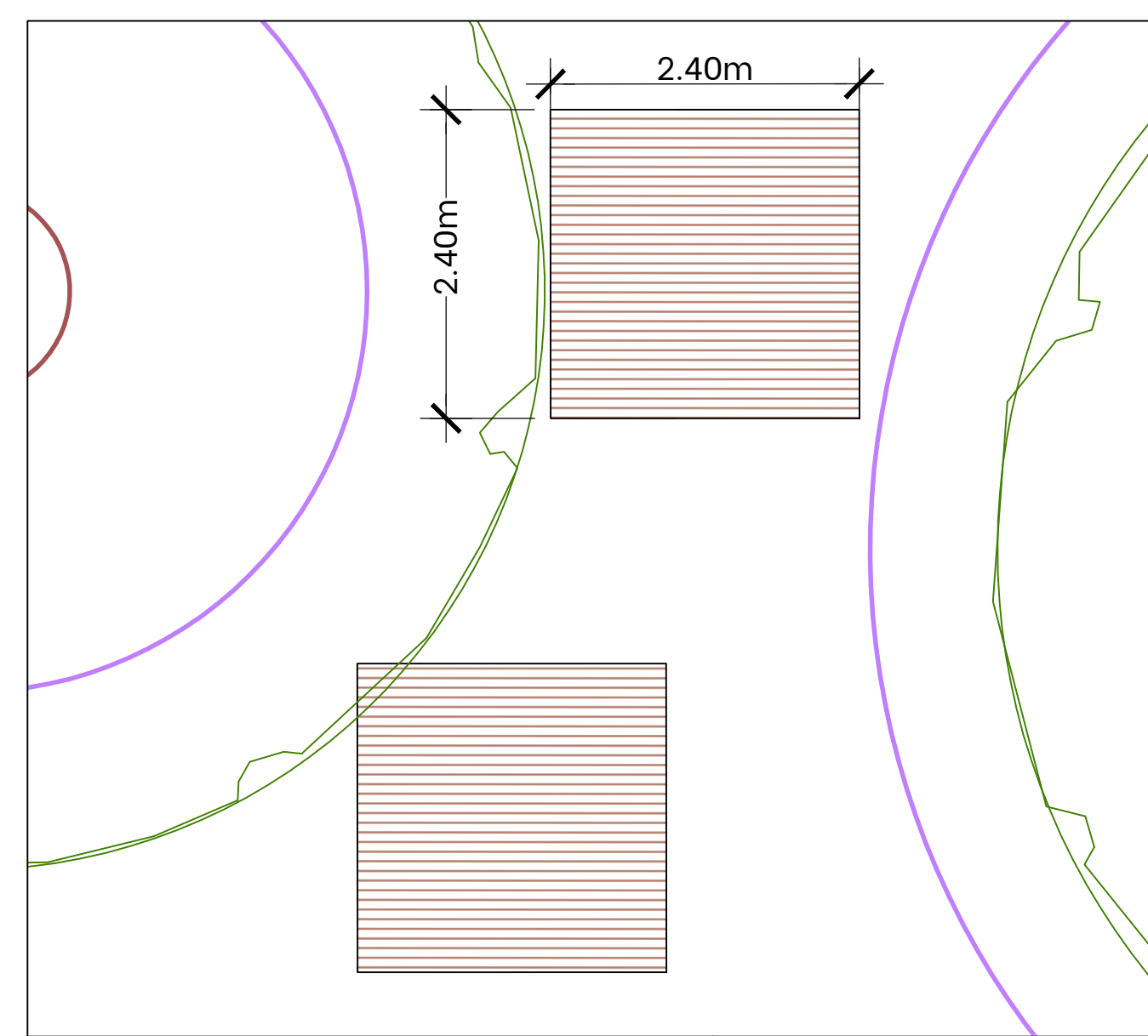
2 FURNITURE - PLATFORM SEATS (No. 2) DETAIL LANDSCAPE PLAN 1:50 @ A1
