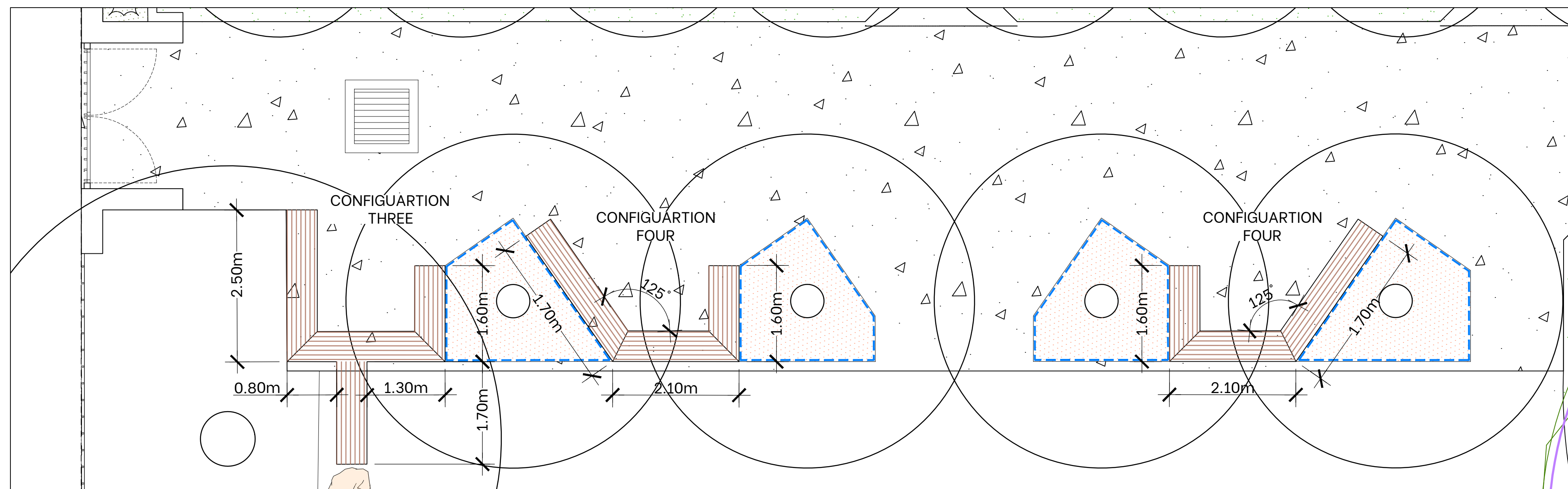
1 BENCH SEATS AT PEDESTRIAN ENTRY DETAIL LANDSCAPE PLAN 1:50 @ A1
